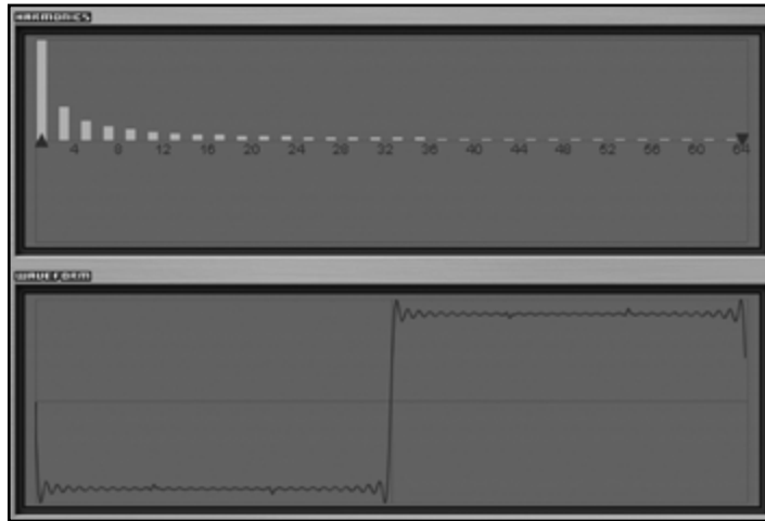
Figure 9.4 An additive square wave.
